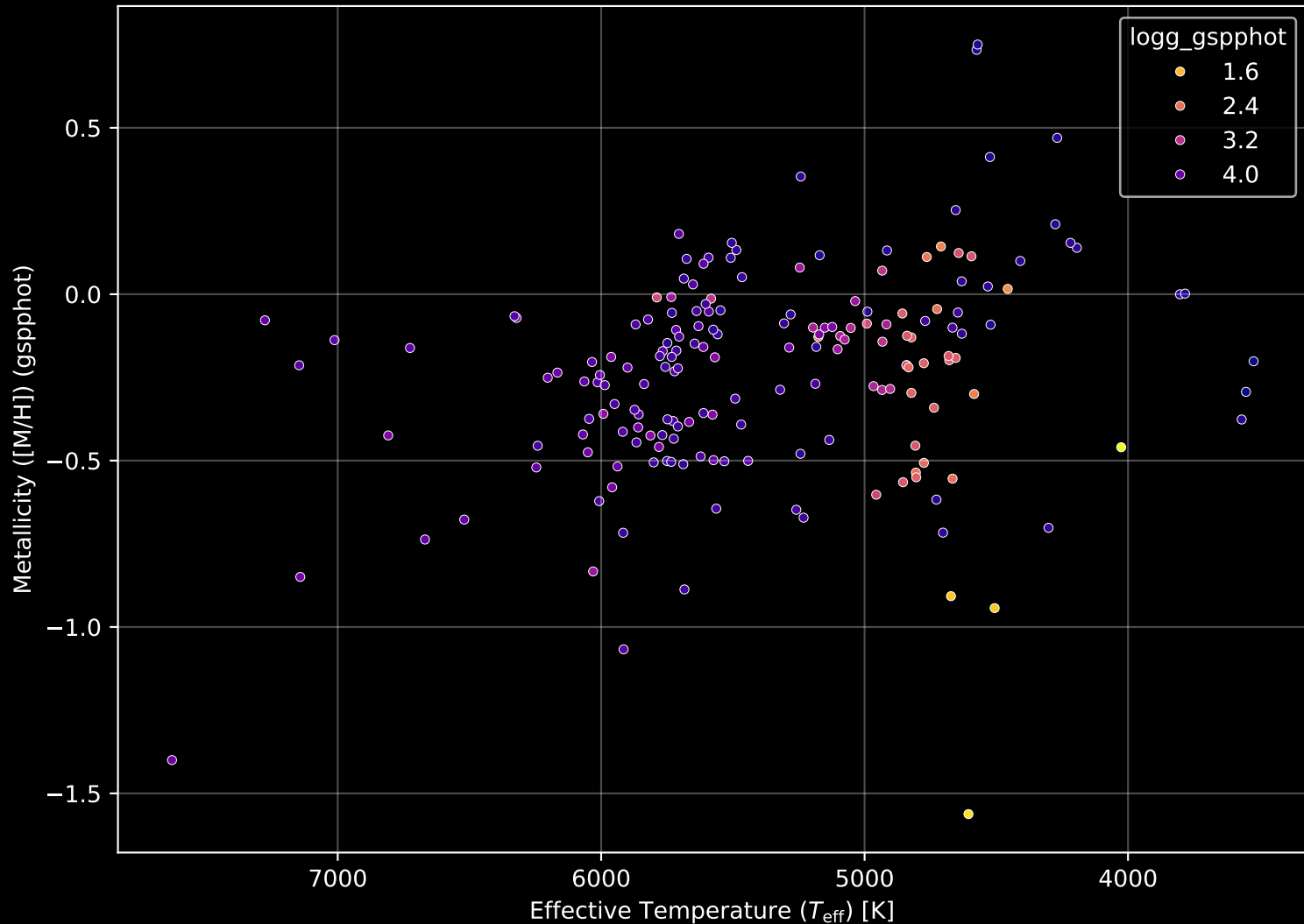
APOGEE DR17 Field: [196+37_MGA] Stellar Population Parameters (n= 183)
