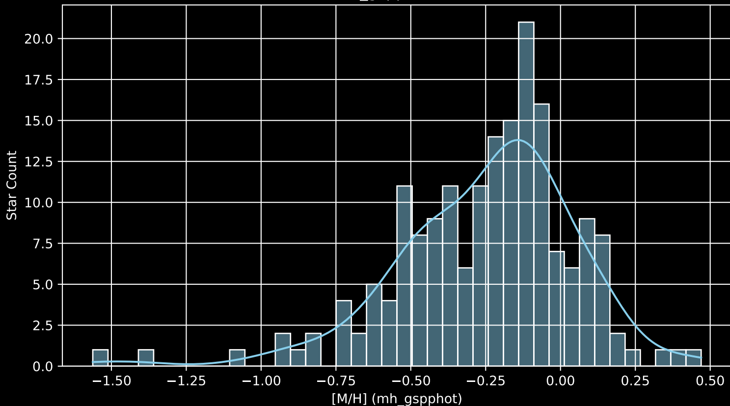
APOGEE DR17 Field: [196+37_MGA [M/H] (mh_gspphot) (n= 181)
