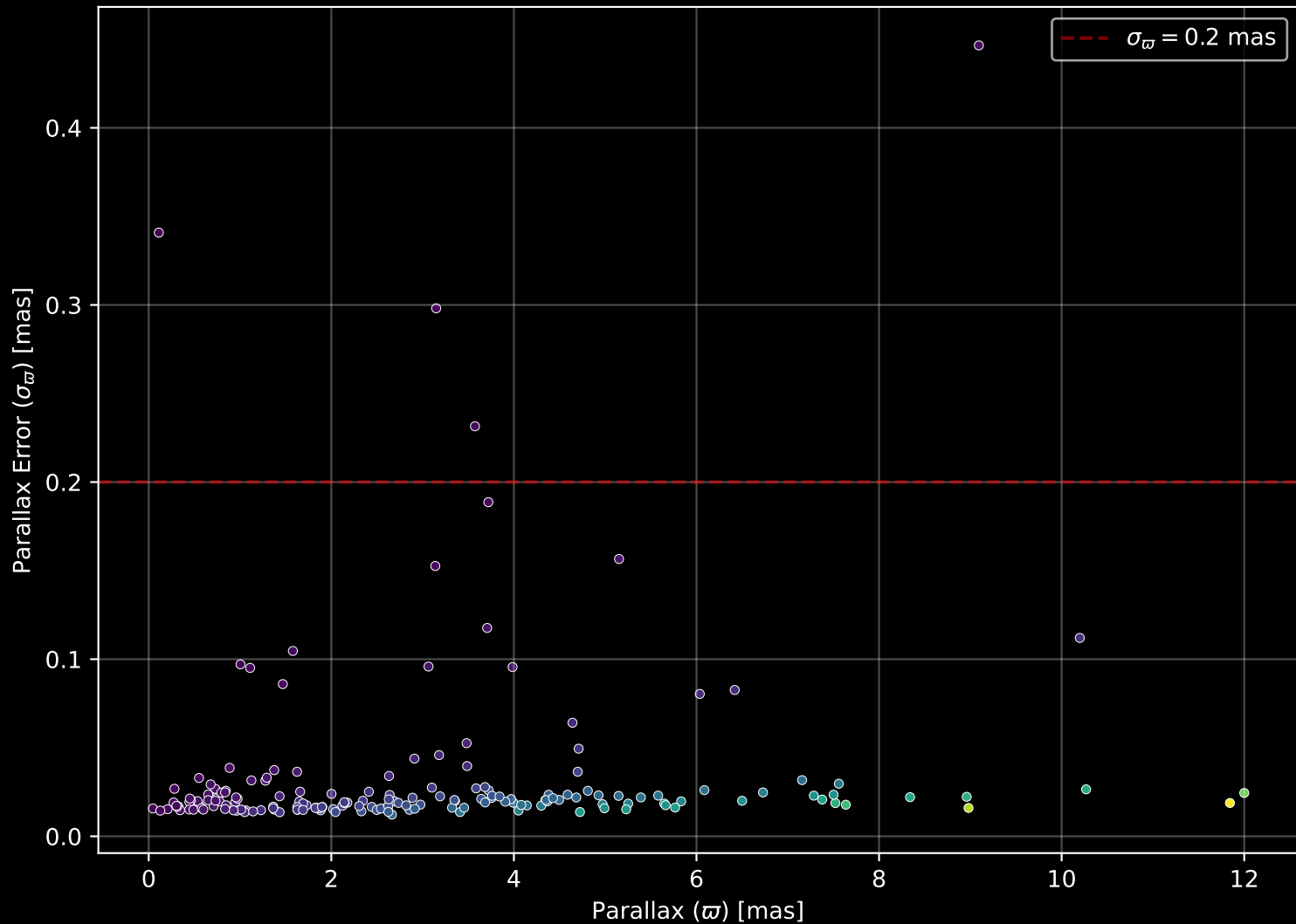
APOGEE DR17 Field: [196+37_MGA] Parallax Quality (n= 183)
