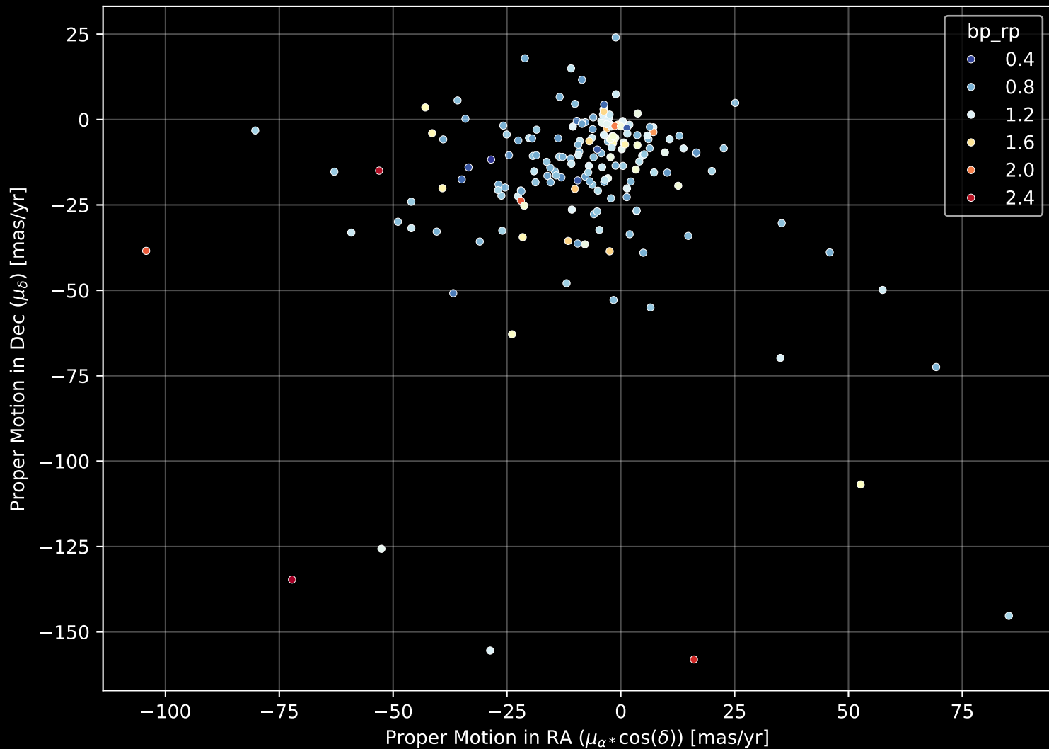
APOGEE DR17 Field: [196+37_MGA] Proper Motion Diagram (n= 183)
