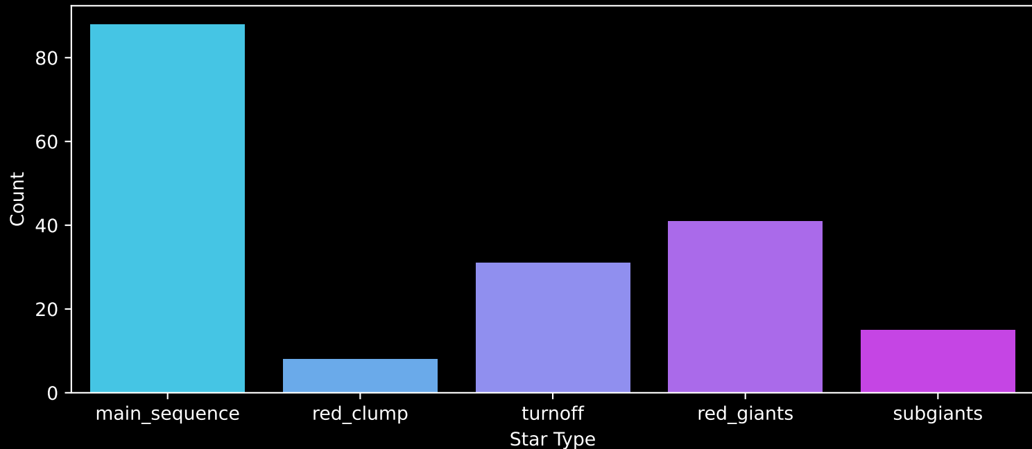
APOGEE DR17 Field: [196+37_MGA] Count plot of Star Type
