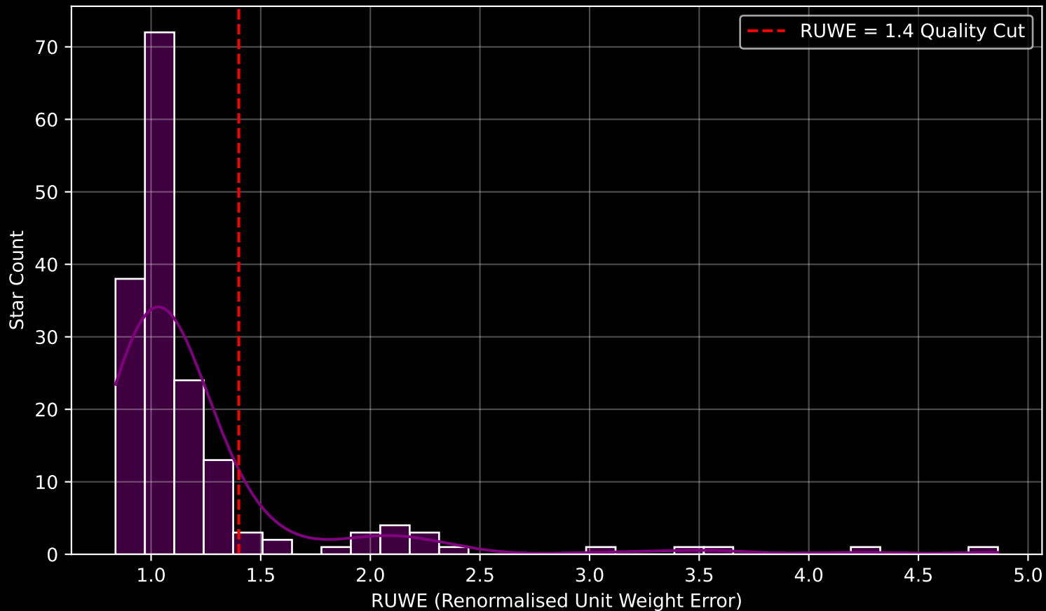
GAPOGEE DR17 Field [196+37_MGA] RUWE Distribution (n= 169)
